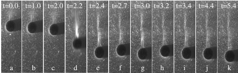
Figure 12: A series of images showing the unstable motion of an aluminum oxide sphere with a sphere-to-tube ratio of a/R = 0.125 and falling with an Weissenberg number of Wi = 3.8 . (Adapted from Figure 8 of Ref. [106])
