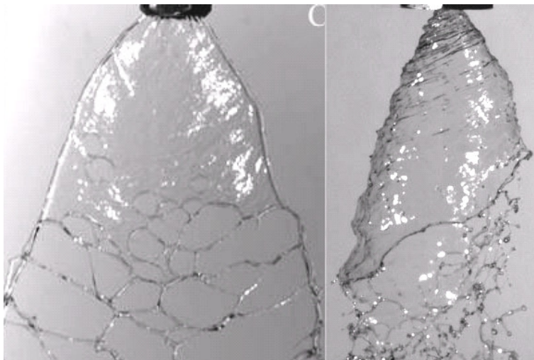
Figure 16: The break-up of sheets of 10mM CTAB/NaSal produced by a 65° flat fan nozzle and a hollow-cone nozzle at Webber numbers We = 1.1 \times 10^4 and We = 2.9 \times 10^3 respectively. (Adapted from Figures 8 and 17 of Ref. [177])
