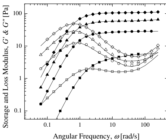
Figure 2: Small amplitude oscillatory rheology of CPyCl/NaSal solutions in 100mM NaCl at T = 20^{\circ}\text{C} . The data include: storage modulus, G' (filled symbols), and loss modulus, G'' (open symbols), for '■' 50/25mM, '●' 100/50mM, '▲' 150/75mM, and '◆' 200/100mM with two-mode Maxwell model fits to each of the data sets (—). (Adapted from Figure 2 of Ref. [23])
