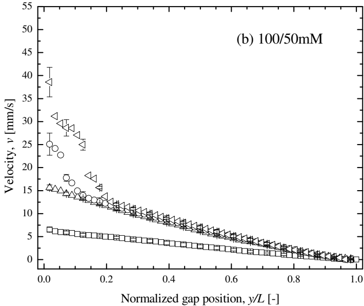
Figure 5: Steady velocity profiles from PIV experiments showing shear band development in a inner-rotating concentric cylinder Couette device with increasing shear rate. The data are for 100/50mM CPyCl/NaSal solutions in 100mM NaCl solution and include shear rates of \dot{\gamma} = 1 \text{ s}^{-1} ( \square ), 3 \text{ s}^{-1} ( \triangle ), 6 \text{ s}^{-1} ( \circ ), and 8 \text{ s}^{-1} ( \triangleleft ). The data show the presence of shear bands above \dot{\gamma} > 3 \text{ s}^{-1} . (Adapted from Figure 8 of Ref. [24])
