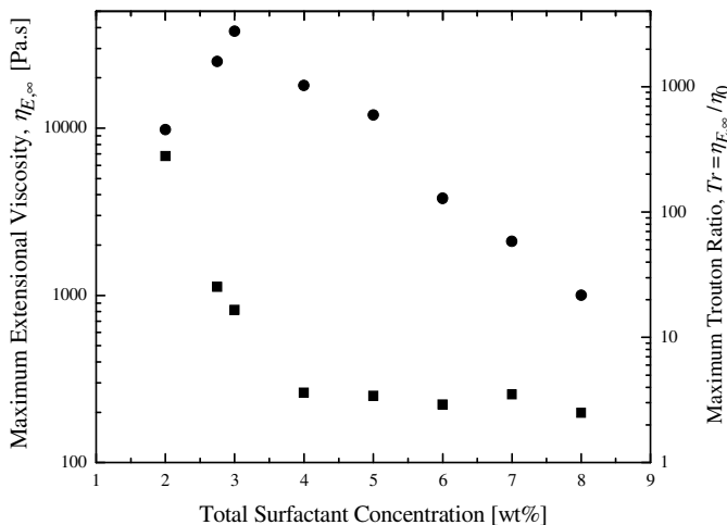
Figure 11: FiSER measurements of the steady-state value of extensional viscosity, ●, and the corresponding Trouton Ratio, ■, as a function of total surfactant concentration for wormlike solutions of 70/30 NaOA/C 8 TAB in water at a constant Weissenberg number of Wi = 3.2 . (Adapted from Figure 10 of Ref. [45])
